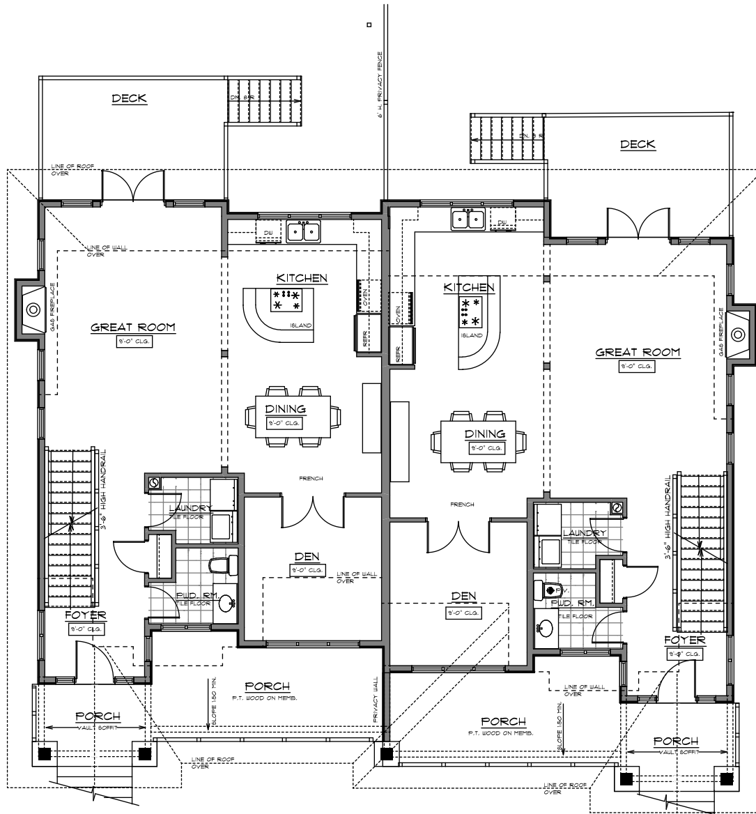
MAIN FLOOR PLAN - SUITE 1 1000 SQ.FT.
